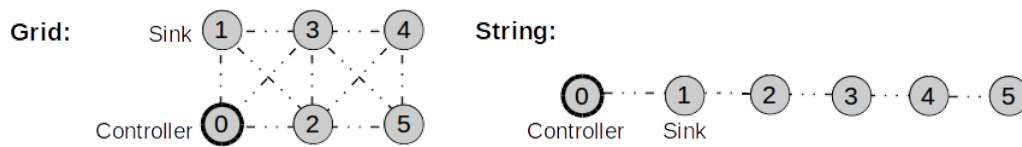
Figure 3. WSN topologies for demonstration
